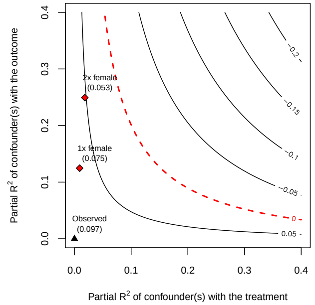
Fig 8: Example of a sensitivity contour plot with benchmarks [ Cinelli et al., 2024a ]. The horizontal axis describes the strength of association of unobserved confounders with the treatment, while the vertical axis describes their association with the outcome. The black triangle shows the original treatment effect estimate, assuming no confounding. Contour lines show a bias-adjusted estimate, assuming confounding with the posited strength, and a direction of the bias that brings the estimate towards zero. The red diamonds show bounds on the strength of unobserved confounders if they were as strong as the observed covariate “female.” In this example, the treatment effect estimate is still robust to unobserved confounding once or twice as strong as “female.”
