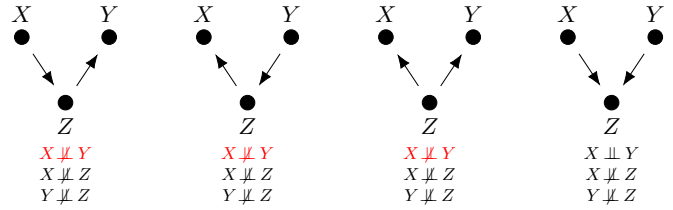
Fig 9: V-structure example: only the rightmost causal structure satisfies all the dependences and independences between the variables X, Y, Z described in the text ( X and Y independent, X and Z dependent, and Y and Z dependent). The statements in red are not consistent with the actual distribution described in the text.
