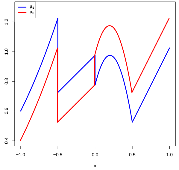
Fig 5: Example regression functions \mu_w(x) = \mathbb{E}[Y_i \mid X_i = x, W_i = w] for which (i) the average causal effect \mathbb{E}[\mu_1(X_i) - \mu_0(X_i)] is zero (e.g., if X \sim \text{Unif}[-1, 1] ), (ii) the individual regression functions \mu_w are non-smooth and difficult to estimate accurately, and (iii) the CATE \mu_1(x) - \mu_0(x) = -0.2 \times \text{sign}(x) is piecewise constant and very simple.
