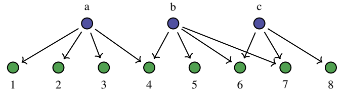
Fig 3: General bipartite interference graph with 3 interventional units (labeled a, b, c) and 8 outcome units (labeled 1, 2, 3, 4, 5, 6, 7, 8).
